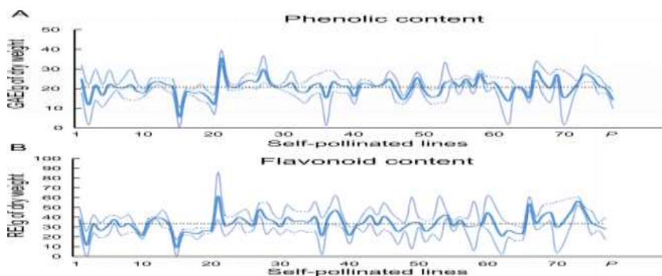
Figure 7. Total phenolic and flavonoid contents measured in M. oleifera parental (P) and 76 self-pollinated lines. (A) Total phenolic content was determined as mg of gallic acid equivalents per gram of dry weight (GAE/g of dry weight). (B) Total flavonoid content was determined as mg of rutin equivalents per gram of dry weight (RE/g of dry weight). Solid lines and dashed blue lines represent the mean and standard deviations (three repeats) respectively. Dashed black lines represent averaged values across the parental and 76 self-pollinated lines.
